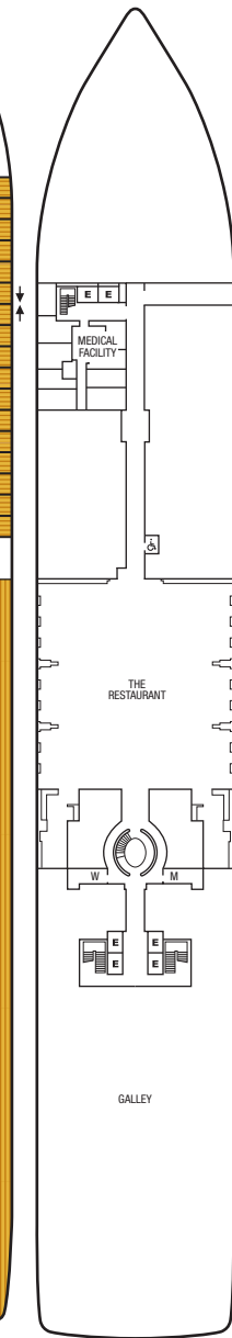
DECK 4
